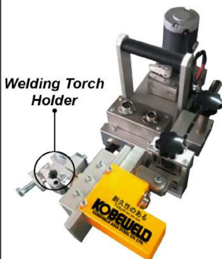
Welding Carriage
